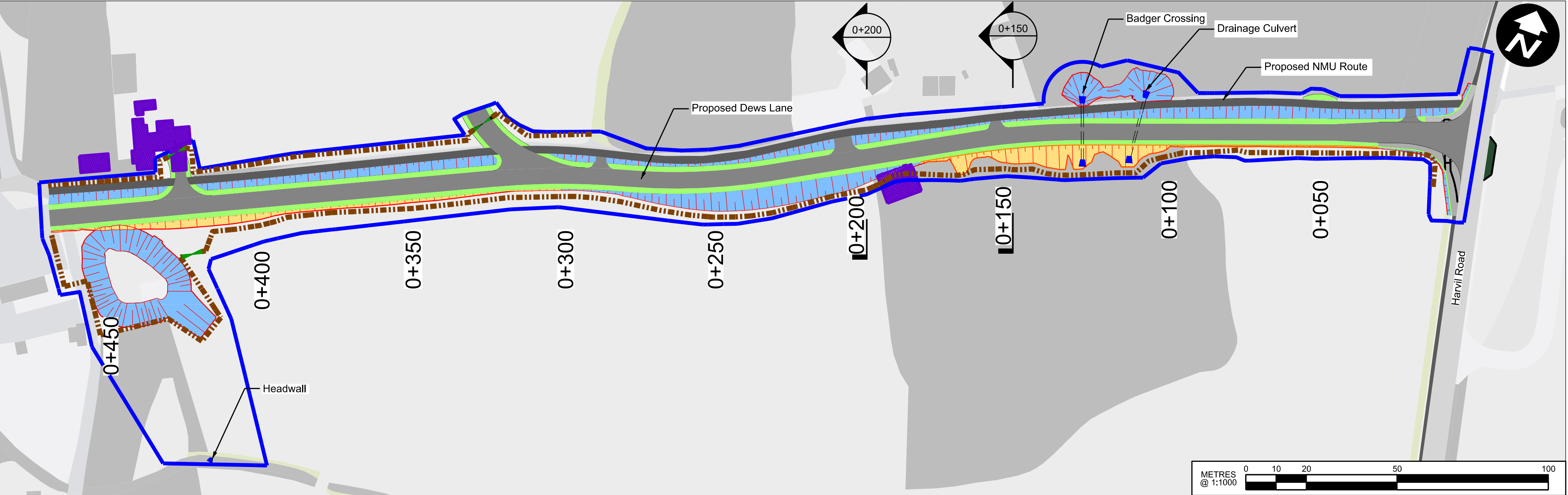
Dews Lane Location Plan Scale 1:1000
